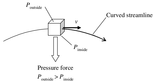
Figure 7. Fluid particle travelling along a curved streamline.
