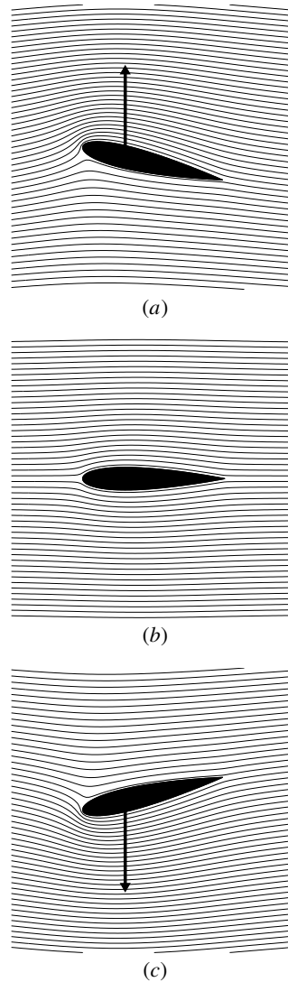
Figure 11. Streamlines around a symmetrical aerofoil at various angles of attack. (a) Positive angle of attack: lift points up. (b) Zero angle of attack: no lift. (c) Negative angle of attack: lift points down.
